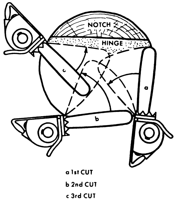
Figure 5-8. Felling cut for large diameter tree.
